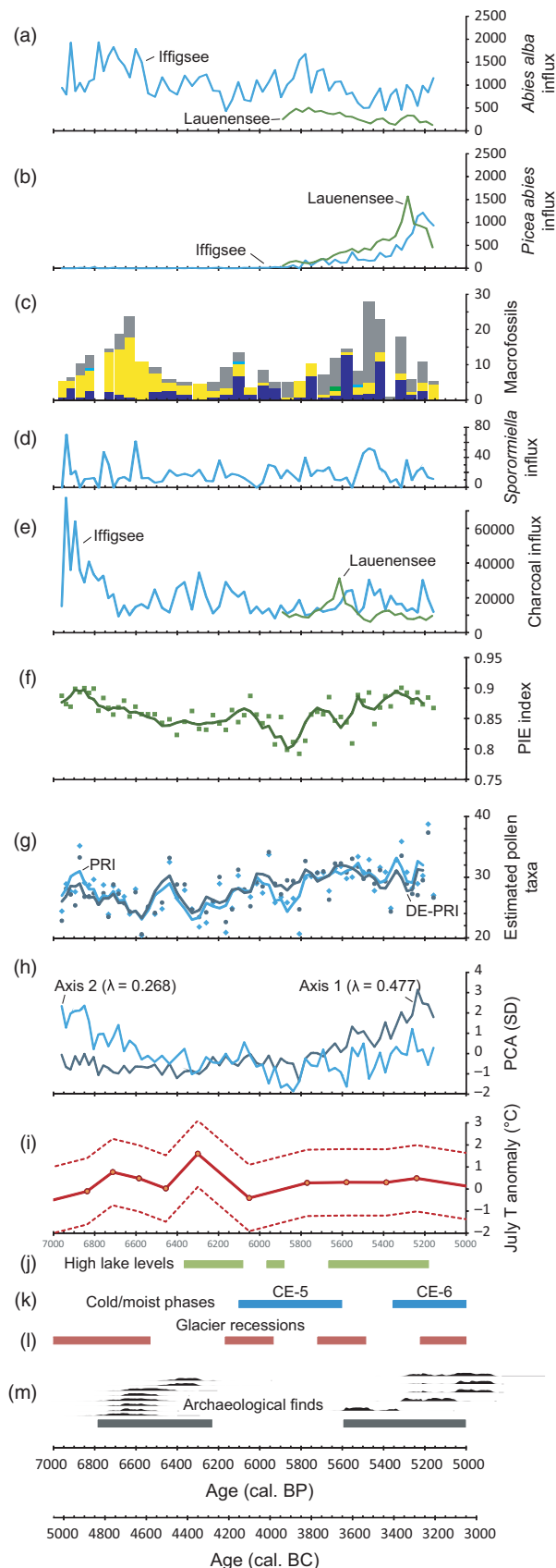
Fig. 5. (a, b) Pollen influx values ( \# \text{ cm}^{-2} \text{ year}^{-1} ) of Abies alba and Picea abies at Iffigsee and Lauenensee, respectively. (c) Stacked macrofossil record of subalpine tree remains at Iffigsee. Blue = Pinus cembra , yellow = Larix decidua , green = Picea abies , light blue = Betula sp., grey = indet. coniferous. (d) Sporormiella influx values at Iffigsee, (e) microscopic charcoal influx at Iffigsee and Lauenensee. Note that the influx curve of Lauenensee is exaggerated by 10× for comparison. (f) Palynological evenness (PIE) and (g) palynological richness (PRI, light blue) as well as evenness-detrended richness (DE-PRI, dark blue) as proxies for biodiversity. The smoothed lines are a three samples running mean. (h) PCA axis 1 and 2. (i) July-temperature anomalies (solid line) from the chironomid-inferred Hinterburgsee temperature reconstruction including root mean square error of prediction (RMSEP; dotted lines) of 1.51 °C (Heiri et al. 2003a). (j) Periods of high lake levels in Central Europe after Magny (2004). (k) Cold and wet phases identified from Central European pollen and macrofossil records after Haas et al. (1998). (l) Glacier recessions in the Swiss Alps indicating warm time periods after Joerin, Stocker & Schlüchter (2006). (m) 14 C-Dates of archaeological finds from the Schnidejoch indicating human presence in the area (Hafner 2012).
