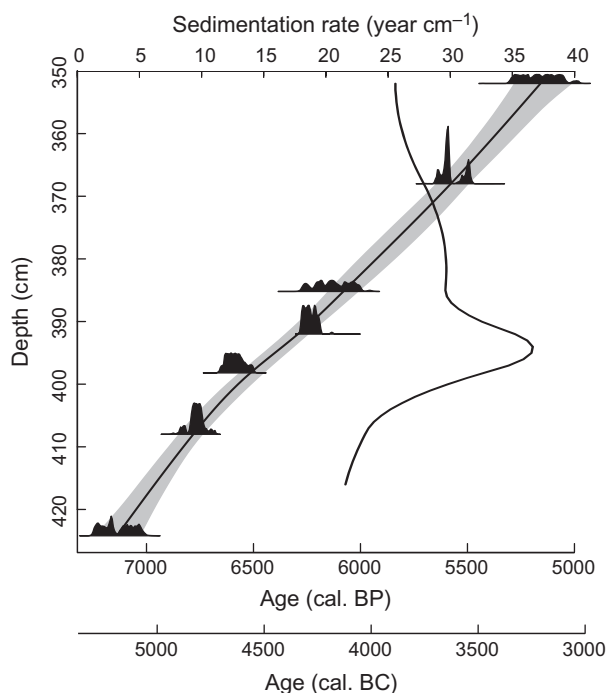
Fig. 2. Age-depth model and inferred sedimentation rate of the Iffigsee high-resolution sediment sequence (352–416 cm). The seven radiocarbon dates used to calculate the age-depth model are shown as probability distributions (small histograms). The 95% confidence interval of the age-depth model (grey area) was calculated with the program clam (Blaauw 2010) by fitting 10 000 smoothing splines to randomly selected dates from the radiocarbon probability distributions. The black line inside the grey area represents the best fit. The vertical solid black curve represents the inferred sedimentation rate.
