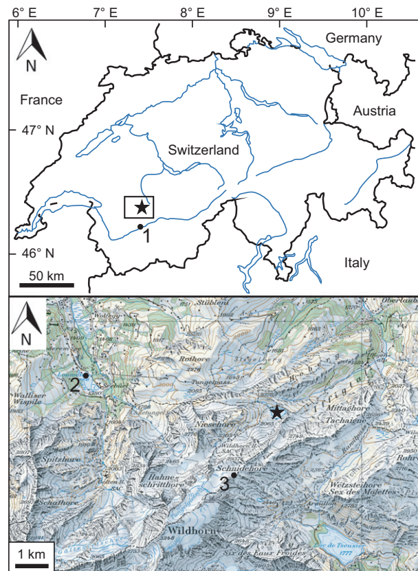
Fig. 1. Map of Switzerland (top) and the study area (bottom) showing the study site Iffigsee at 2065 m a.s.l. (star) and other important sites in the region: 1. Neolithic settlements at Sion (Curdy 2007), 2. Lauenensee (1382 m a.s.l.), 3. the archaeological site and mountain pass Schnidejoch (2765 m a.s.l.). Map reproduced by permission of Swisstopo.
