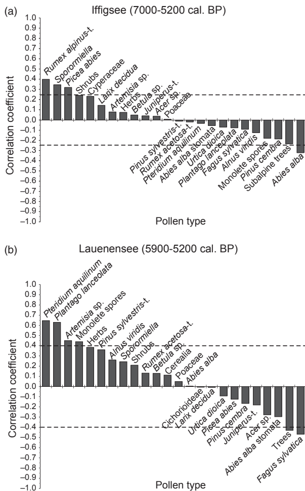
Fig. 8. Correlograms showing correlation coefficients between microscopic charcoal influx and selected pollen and spore types for (a) Iffigsee and (b) Lauenensee. The dashed lines mark the significance level ( P < 0.05 ).
