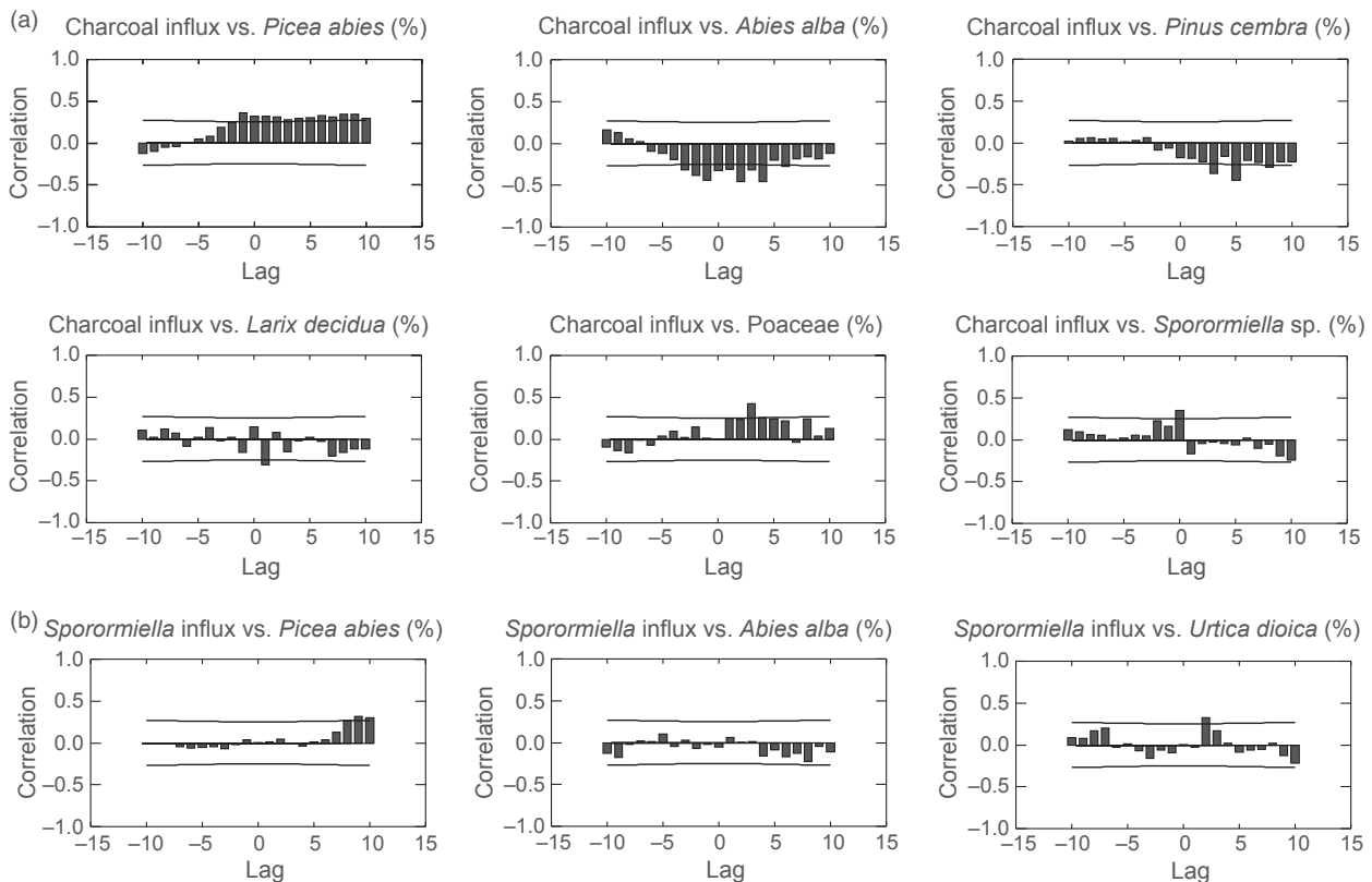
Fig. 7. Cross-correlation analysis of (a) microscopic charcoal influx and (b) Sporormiella influx vs. selected taxa from the high-resolution sequence (6960–5160 cal. BP). 1 lag = 29 ± 7.5 years. The solid black lines mark the significance level ( P < 0.05 ). [Correction added on 12th February 2015, after first online publication: missing labels added to Figs 7 and 8]
