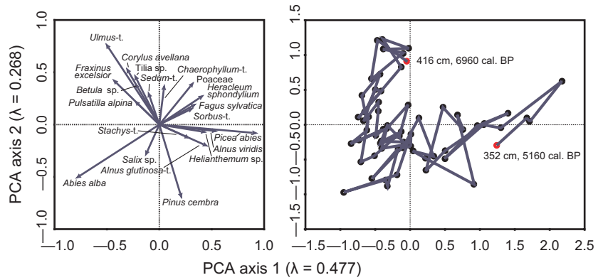
Fig. 6. PCA scatterplots of (left) species and (right) sample scores. The first axis explains 47.7% of the variance in the data set and the second axis 26.8%. Subalpine tree species are printed in bold.
